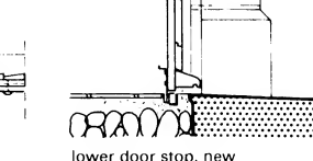
⑬ New oak door drip on old wooden frame
